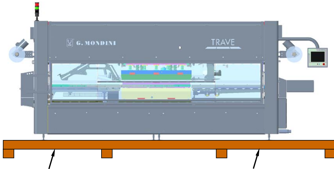
Figure 4-1: Lifting using a forklift truck.
